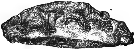
PALÆOPHIS TOLIAPICUS. ( Ophidian of the Eocene. )
